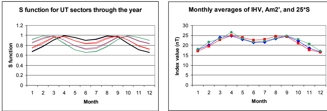
Figure 9. (a, Left) Monthly average values of the function S(\Psi) (eq. (3)) for eight six-hour UT intervals: 00-06 h , 03-09 h , 06-12 h , ..., 21-03 h . Due to symmetries there are only half as many different curves. The curves for 00-06 h (for which IHV is calculated for the 290°E longitude sector) and for 03-09 h are shown as heavy black lines. The curves for 06-12 h and 21-03 h are shown in red, for 09-15 h and 18-24 h in purple, and for 12-18 h and 15-21 h in green. (b, Right) Monthly average variation through the year of IHV^H for 1901-2001 (blue), of Am2' , for 1959-2001 (green), and of 25 nT times \langle S(\Psi) \rangle (red, corresponding to the black curves in the left panel).
