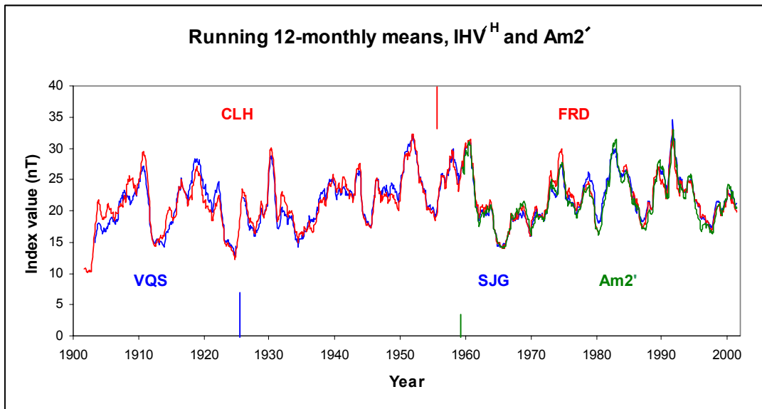
Figure 7. Running 12-monthly means of calibrated IHV^H for Cheltenham (CLH, red; before 1956.0), Fredericksburg (FRD, red; after 1956.0) and Vieques (VQS, blue; before 1925.0) and San Juan (SJG, blue; after 1926.0). For comparison Am2' = 0.8 Am2 + 4 is shown in green since 1959.0. Often the curves fall on top of each other and it can be hard to distinguish between them. This is good.
