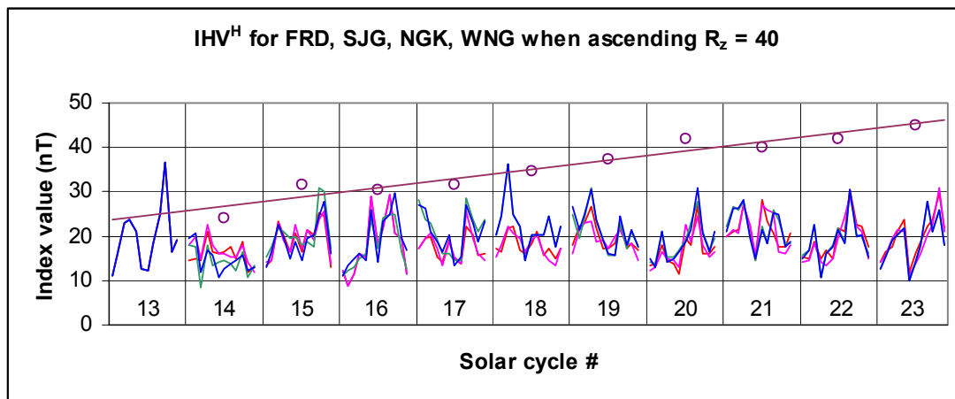
Figure 10. Comparison of four IHV series for the years (monthly values centered on 1891.5, 1904.5, 1915.5, 1925.5, 1935.5, 1945.5, 1955.5, 1966.5, 1977.5, 1987.5, 1998.0) in the ascending phase of each solar cycle since 1890 where the yearly average sunspot number was R_z \approx 40 . In most years, a semiannual variation is discernible. The differences between the curves are mostly real, reflecting the longitude difference between the American (FRD and SJG) series and the European series (NGK and WNG). The FRD series (CLH, FRD) is shown in red, the SJG series (VQS, SJG) in orange, the NGK series (POT, SED, NGK) in blue and the WNG series (DBN, WIT, WNG) in green. Often the curves cover each other. Open circles (with trendline) show the open flux (in units of 10^{13} Wb) calculated by Lockwood et al. [1999] for these years.
