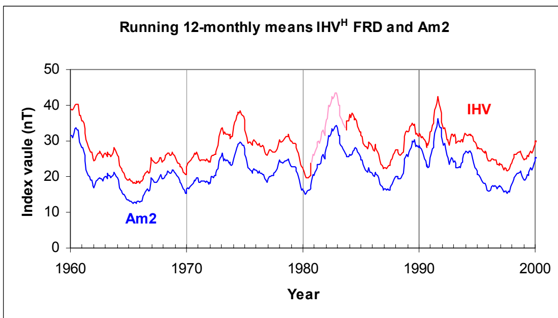
Figure 4. (Top) Monthly means of the IHV -index (red) for the H-component at Fredericksburg and the Am2 -index (blue) for the interval 1960-1999. The year-labels mark the beginning of the year. (Bottom) 12-month running mean of the same data. The missing data (1980.5-1984.0) is filled-in using the relationship IHV (filled-in) = 1.26 \cdot Am2 (from Figure 3) and shown in lighter color. The filling-in was done to preserve to “flow” of the curve.
