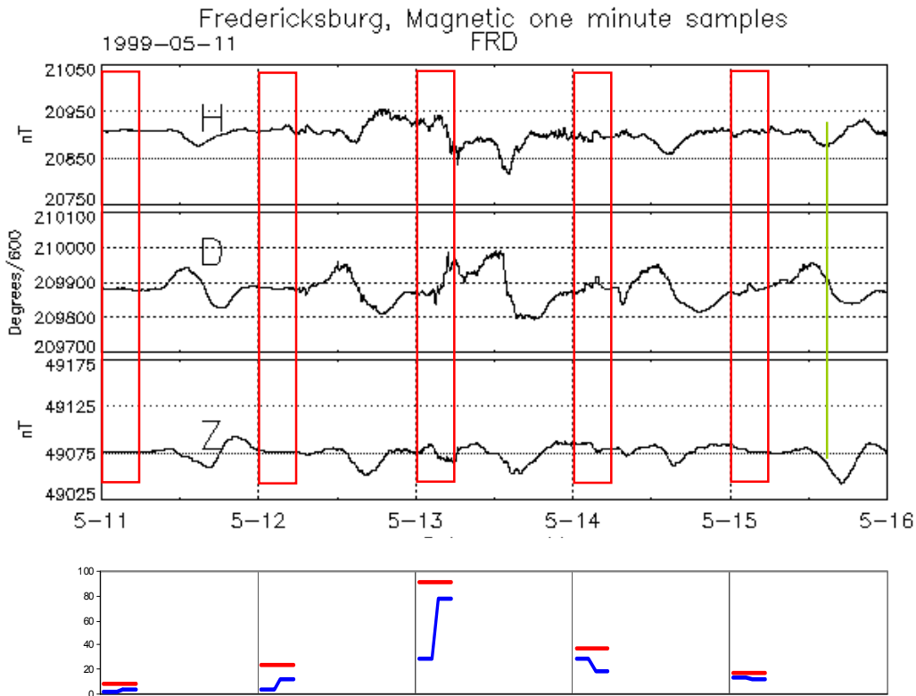
Figure 1. (Top) Variation of the geomagnetic elements at Fredericksburg May 11-15, 1999 (UT). The “effective” noon is marked with a green line on May 15. The red boxes indicate the six hours around midnight where the regular variation is absent or minimal. These intervals are used to define the IHV -index. May 11 is a good example of a day with very little activity. It is, in fact, the famous day where “the solar wind disappeared”. The solar wind momentum flux was only 1% of its usual value and the magnetosphere diameter was five times larger. The interplanetary magnetic field was not affected and had its usual properties. The variability of S_R is clearly seen by comparing May 11 and May 15. (Bottom) The am -index (blue) for these six-hour intervals and the IHV^H -index (red) calculated for each interval.
