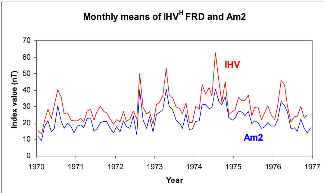
Figure 2. Comparison of monthly means of the IHV -index (red) calculated for the H-component at Fredericksburg and the Am2 -index (blue) for the interval 1970-76. The year-labels on the abscissa mark the beginning of each year.
