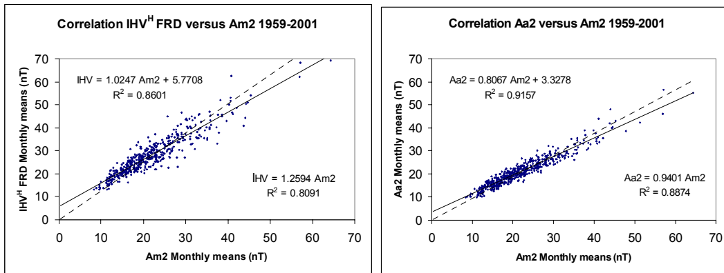
Figure 3. (Left) Linear correlation between the 467 monthly means of data of IHV^H at Fredericksburg where more than twenty days of data were available in each month versus corresponding monthly means of the am -index calculated using only the 00-03 and 03-06 three-hour UT-intervals. (Right) Linear correlation between monthly means of the aa -index versus monthly means of the am -index for these same three-hour intervals and months. The dashed lines show the correlations when forced through the origin.
