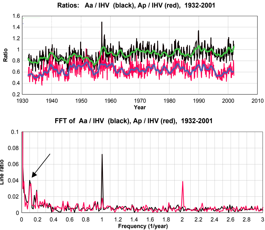
Figure 12. (Top) Ratios of monthly means of Aa/IHV (black) and of Ap/IHV (red) for the interval 1932-2001. We are using the combined IHV series and Aa and Ap over the same UT intervals. 12-monthly running means are shown as heavy curves. (Bottom) FFT frequency spectra of the above ratios. The arrow points to a solar cycle peak.
