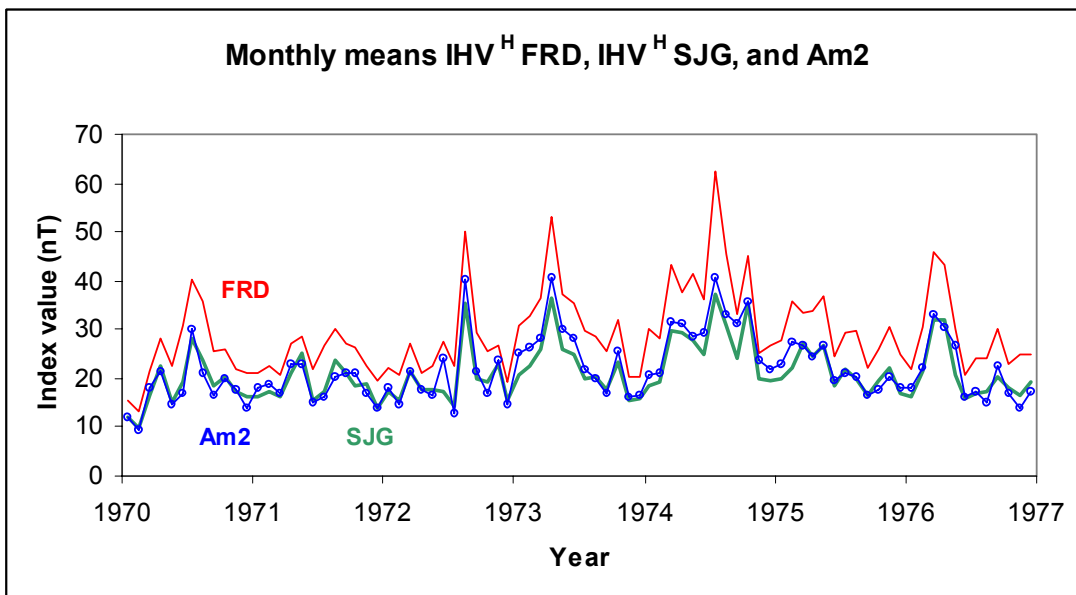
Figure 6. Monthly means of IHV^H for Fredericksburg (red), San Juan (green), and Am2 (blue with circles) for the interval 1970-76.
