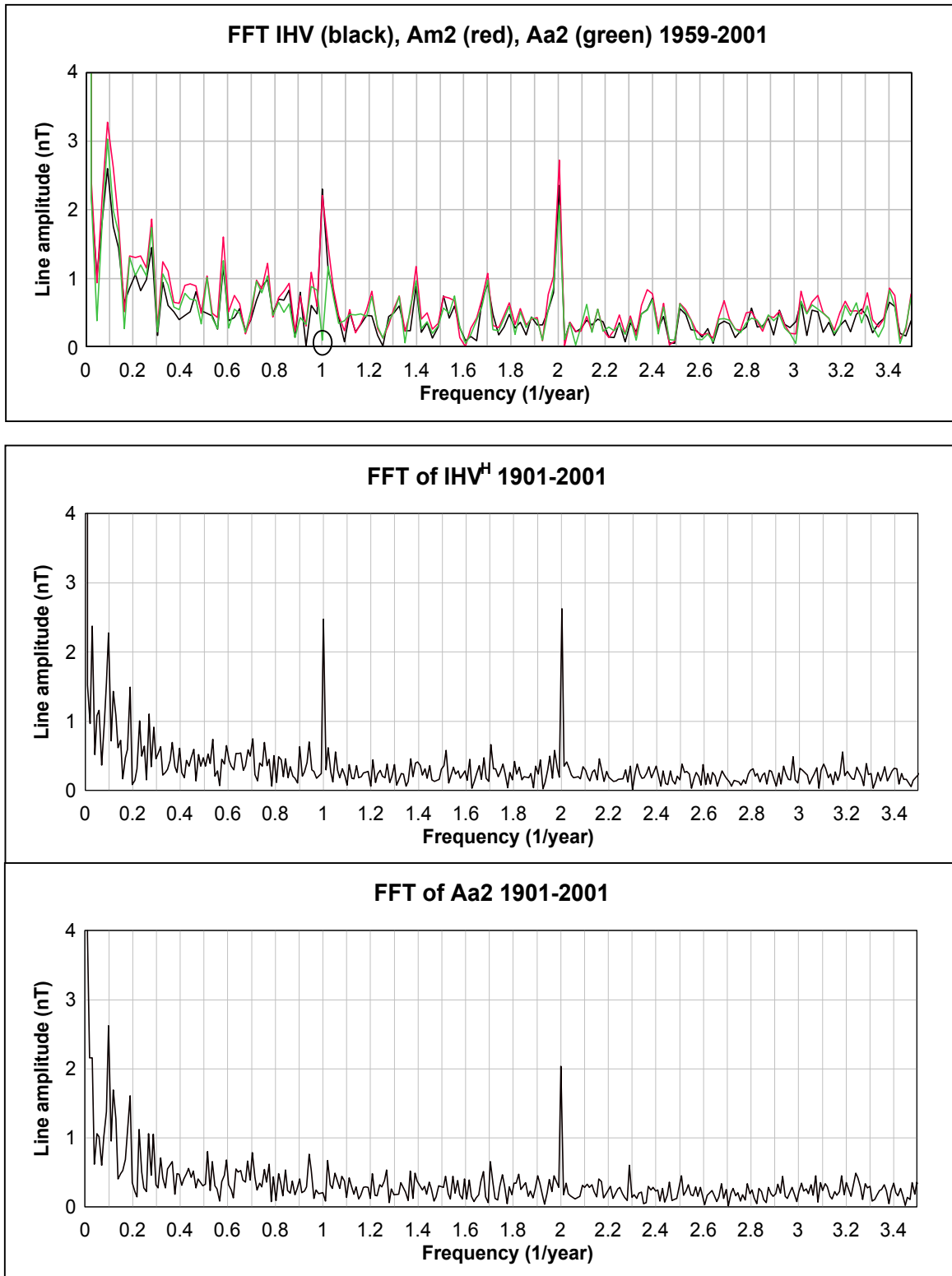
Figure 8. FFT frequency spectra of (top) IHV^H (black), Am2 (red), and Aa2 (green) for 1959-2001. (Bottom) IHV^H and Aa2 for 1901-2001.
